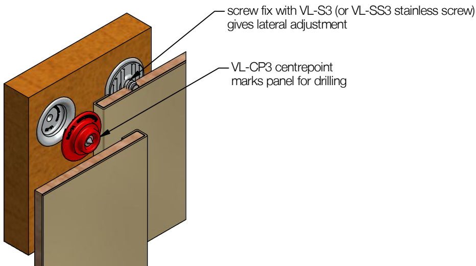
3 Exploded view showing center point marker, install option
