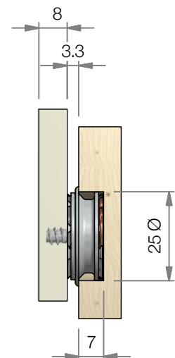
4 Section through recessed installation
