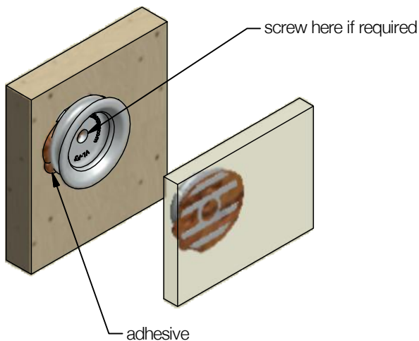
3 Exploded view showing center point marker, install option
