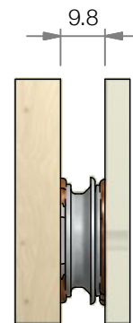
2 Section through installed clip
